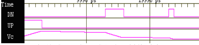
Fig. 13. CP-LPF SystemC-AMS Model Simulation
