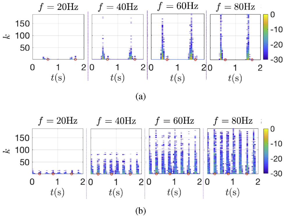
Fig. 4. Normalized energy in dB in the joint graph and short-time Fourier transform domain. (a) Sinus rhythm; (b) atrial fibrillation. The scalar k represents the graph frequency index, t(s) the time in seconds, and f the temporal frequency. Each plot shows the spatial distribution of the signal energy as a function of time; different plots refer to different temporal frequencies. The red circles mark the peak of the ventricular activity. (For interpretation of the references to color in this figure legend, the reader is referred to the web version of this article.)
