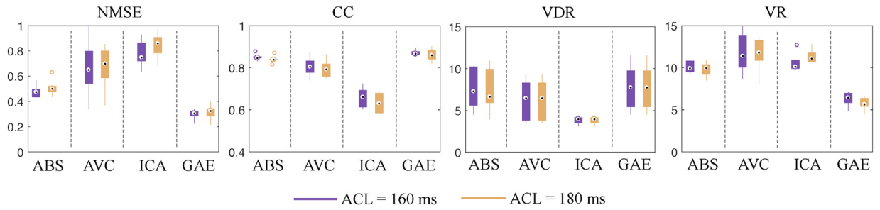
Fig. 7. Boxplot performance on synthetic data of the average beat subtraction (ABS) [28], adaptive ventricular cancellation (AVC) [29], independent component analysis (ICA) [29], and the proposed graph-based atrial activity extraction (GAE) method. Two atrial cycle length (ACL) of 160 and 180 ms are considered. The proposed GAE method achieves the lowest normalized mean square error (NMSE) and ventricular residue (VR), and highest correlation coefficient (CC) and depolarization reduction (VDR) in both cases. The boxplots of NMSE, CC, and VR for the GAE method are comparatively short, which suggest that the GAE performance is more stable. Similar condensed boxplots are also observed for the ABS, but it presents outliers in the plots of NMSE and CC.
