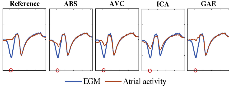
Fig. 8. Illustrative example of the synthetic epicardial electrogram (EGM), synthetic pure atrial activity (AA) and the estimated atrial activity by the different algorithms. The left plot shows the synthetic EGM (blue) and the synthetic atrial activity (red). The other plots show the synthetic EGM (blue) and the estimated atrial activity (red) with different algorithms: average beat subtraction (ABS) [28]; adaptive ventricular cancellation (AVC) [29]; independent component analysis (ICA) [29]; proposed graph-based atrial activity extraction (GAE). The red circles mark the peak of the ventricular activity determined by the ECG measurements. (For interpretation of the references to color in this figure legend, the reader is referred to the web version of this article.)
