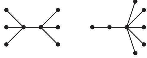
Fig. 1. Two cospectral trees with the same number of edges. With respect to the adjacency matrix, almost all trees are non determined by their spectrum. Both graphs have the same characteristic polynomial t^4(t^4 - 7t^2 + 9) , hence cospectral.
