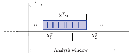
FIGURE 7: A single symbol spread by the block code, shifted over \tau with respect to the beginning of a data packet.
