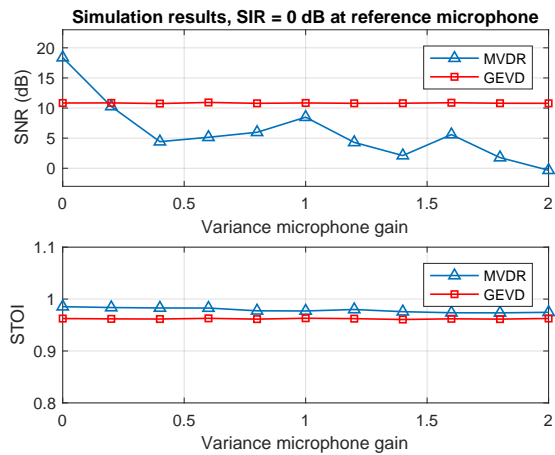
Fig. 2. SNR/STOI scores vs. variance of the gain.
