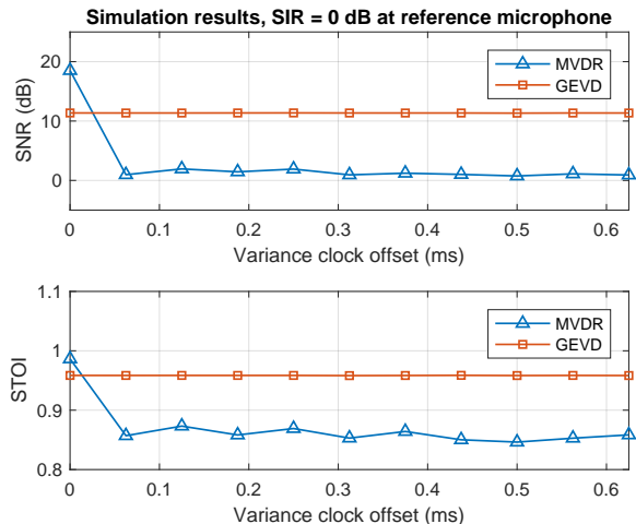
Fig. 1. SNR/STOI scores vs. variance of the clock offset.
