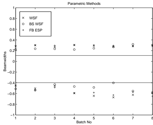
Figure 11: Parameter estimates for the WSF method in element-space and beamspace, and for the ESPRIT algorithm with forward-backward averaging. The methods are applied to the 12.34 GHz data. The vertical axis is normalized by the beamwidth and the horizontal axis indicates the batch number. “True” DOAs are indicated by horizontal lines.
