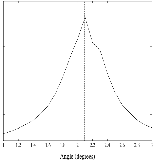
Figure 17: Estimation of orientation of the line in Figure 16, using TLS ESPRIT (vertical line) and the Hough transform. The peak magnitude of Hough Transform yields a similar orientation as TLS ESPRIT
