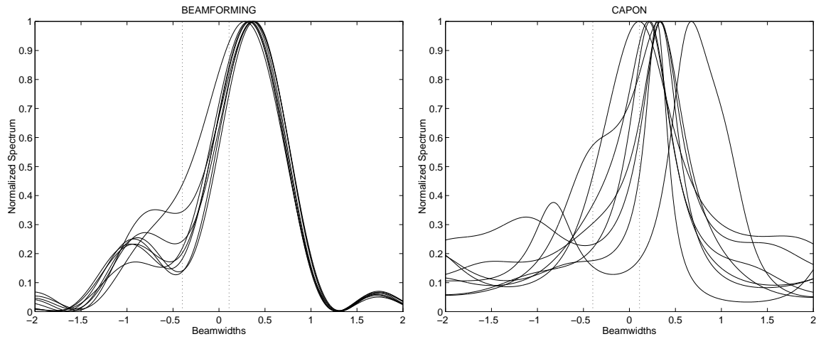
Figure 8: Spatial spectra for the beamforming (left) and Capon (right) methods. The results from the 8 batches of the 12.34 GHz data are overlaid. The horizontal axis contains the electrical angle in fractions of the beamwidth. “True” DOAs indicated by vertical dotted lines.
