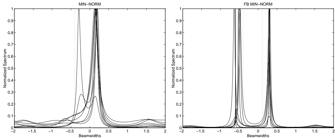
Figure 10: As in Figure 23, but for the Min-Norm method, with (right) and without (left) forward-backward averaging.
