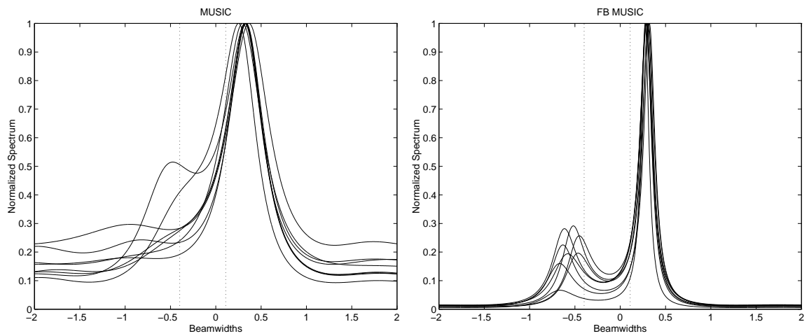
Figure 9: As in Figure 23, but for the MUSIC method, with (right) and without (left) forward-backward averaging.
