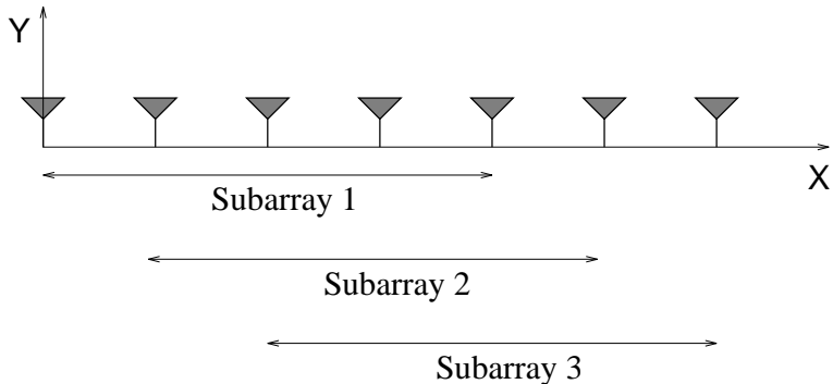
Figure 6: Spatial smoothing means that the array is split into identical subarrays, the covariances of which are averaged.
