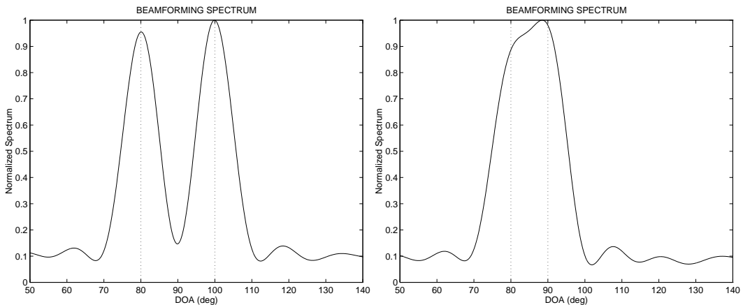
Figure 4: Normalized beamforming spectra versus DOA for two different scenarios. True DOAs indicated by dotted vertical lines.
