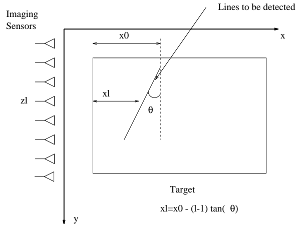
Figure 15: Typical linear array setup of photosensors for detection of lines (defects) in a manufacturing environment, by merely using the geometry and modeling the pixel responses as cisoids.
