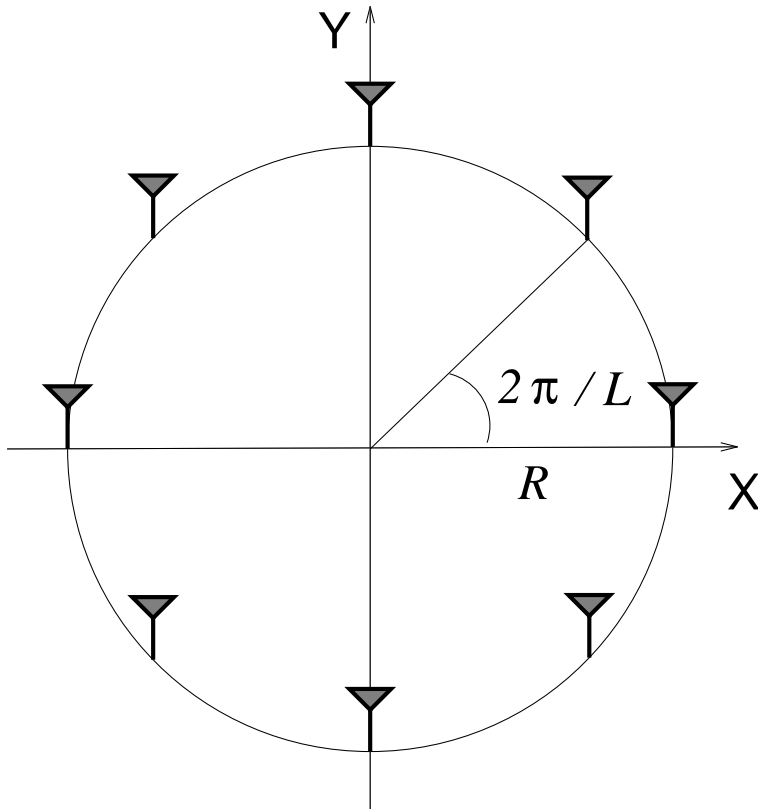
Figure 3: Uniform Circular Array geometry
