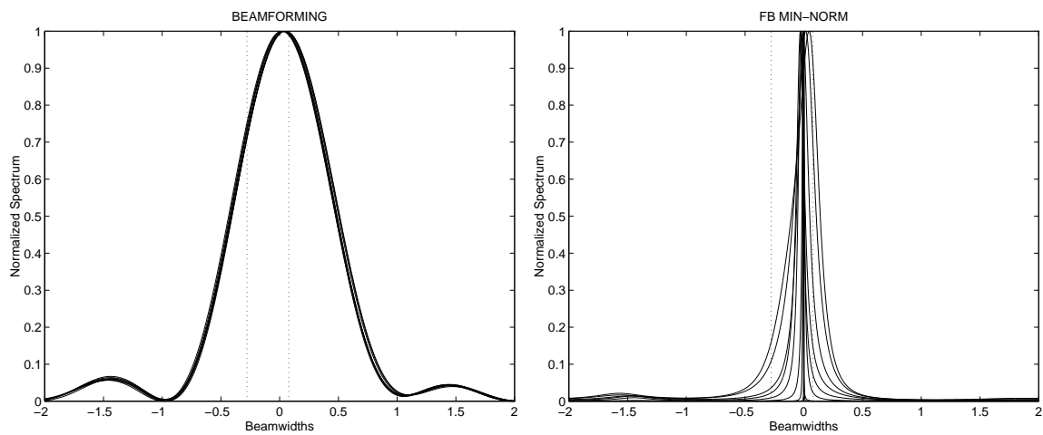
Figure 12: Spatial spectra for the beamforming (left) and FB Min-Norm (right) methods applied to the 8.62 GHz data.
