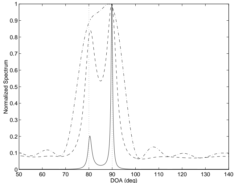
Figure 5: Normalized spectra versus DOA for two different scenarios. The dash-dotted curve represents the conventional beamformer, the dashed curve is Capon's method and the solid curve is the "MUSIC spectrum". True DOAs indicated by dotted vertical lines.
