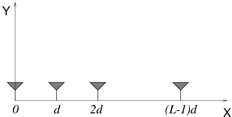
Figure 2: Uniform Linear Array geometry
