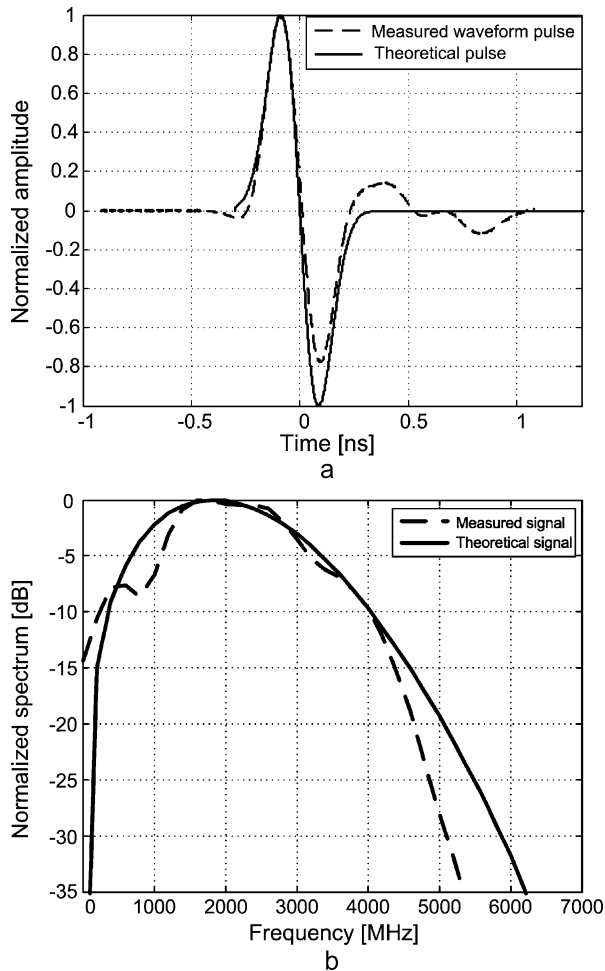
Fig. 15. Measured output waveform from the pulse generator and its approximation with the first derivative of Gaussian pulse: (a) time domain and (b) frequency domain.
