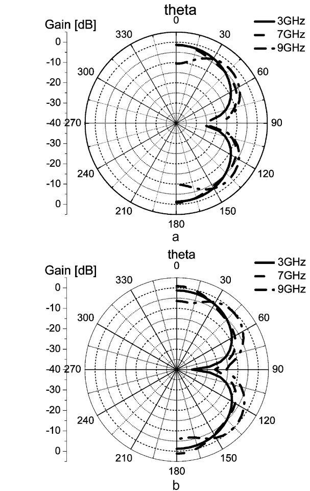
Fig. 7. Antenna radiation patterns (in dB) in E-plane for (a) infinite and (b) finite dielectric substrate.
