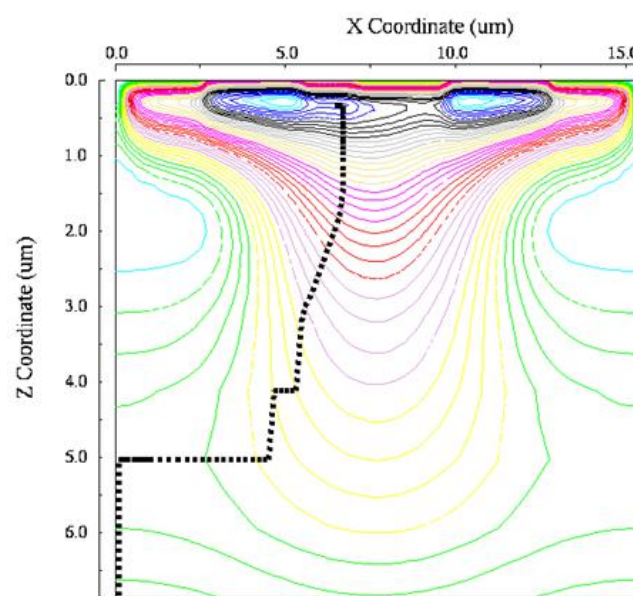
Figure 13. Selective collection of an electron generated at the “left” corner by the “left” collection gate ( 0 < z < 6.9 \mu\text{m} ).
