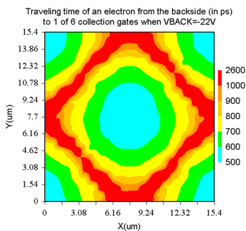
Figure 16. Traveling time of an electron from a point of the backside to 1 of 6 collection gates (ps) (Backside voltage -22 \text{ V} ).
