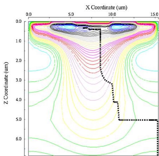
Figure 15. Traveling time of an electron from a point of the backside to 1 of 6 collection gates (ps) (Backside voltage -32 \text{ V} ).
